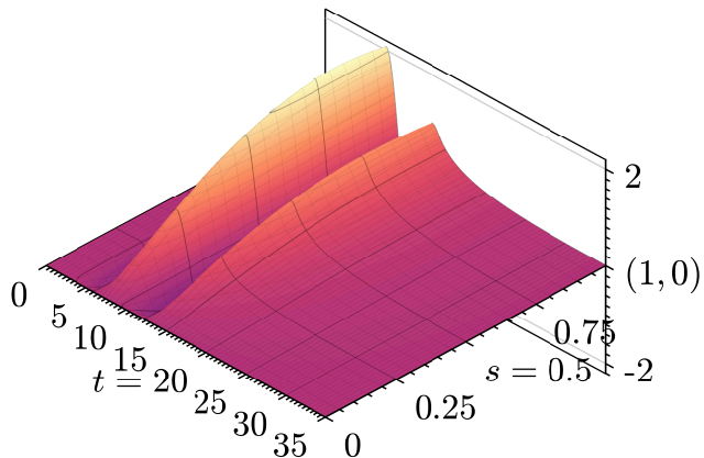
(b) Closed-loop response
